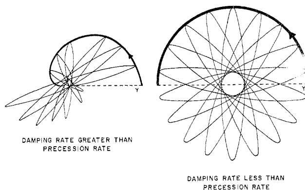
Figure 3. The orbit of an electron initially excited along the y axis executing Larmor precession about a magnetic field perpendicular to the plane of the figure. Shown is one half-turn. Note that the degree of polarization of the fluorescent light is controlled by the competition between the rate of spontaneous emission and the rate of Larmor precession (from Hanle 11 ).
